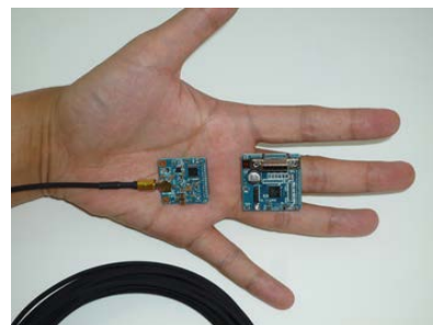
roboVIEW for Camera Link 変換アダプタ
